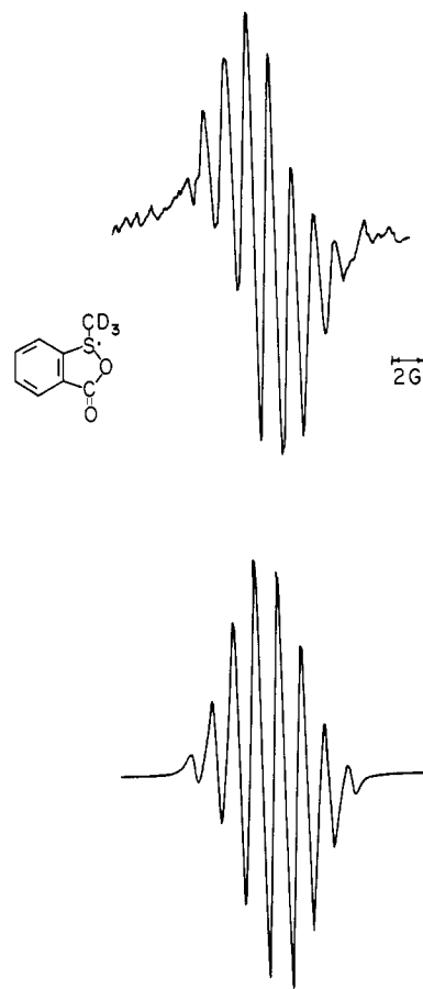
Figure 4. Top: ESR spectrum obtained for the photolysis of tert -butylperoxy 2-((trideuteriomethyl)sulfonyl)benzoate in methylene chloride solution at -85^\circ\text{C} . Bottom: Computer-simulated spectrum using a_{3\text{H}} = 1.4 G, a_{\text{H}} = 1.5 G, and \Delta H_{\text{pp}} = 0.5 G.
